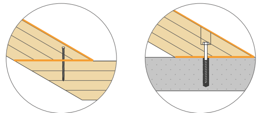
03 Stair-landing departure connection
