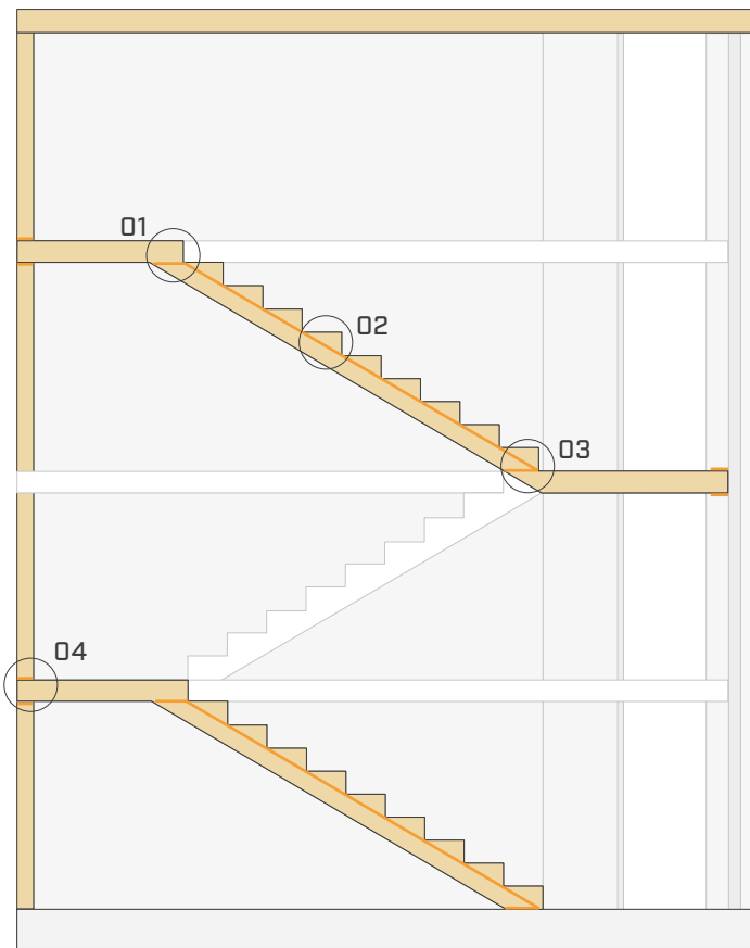
Explanatory section of timber staircase.
