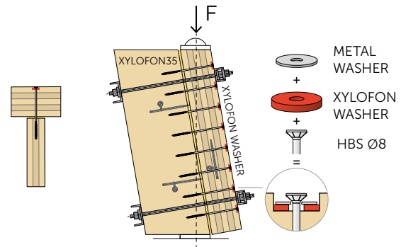
TEST [ T-X-W ] (CLT - XYLOFON35 + XYLOFON WASHER - CLT)
