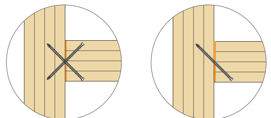
04 Landing-passing wall connection
