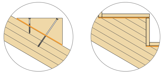
02 Step-stair structure connection
